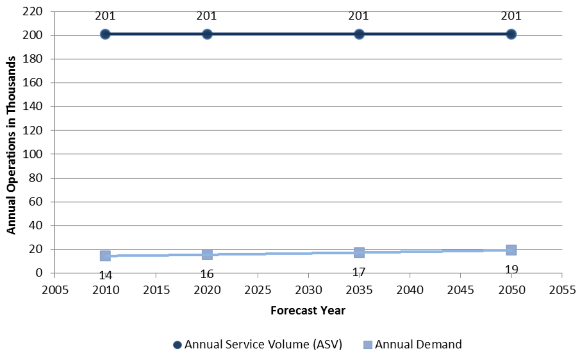
Exhibit C-1: Dade-Collier Training and Transition Airport - Airfield Demand-Capacity Comparison
